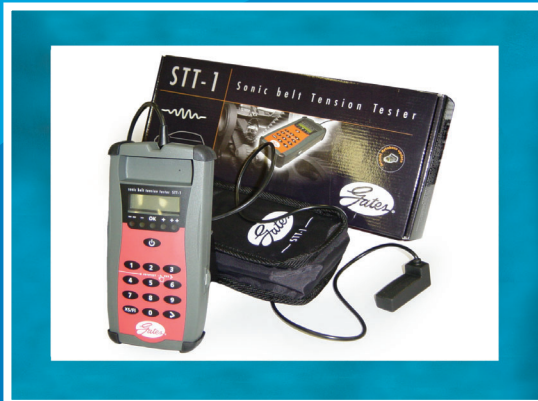
SONIC BELT TENSION TESTER. PART No. STT-1
